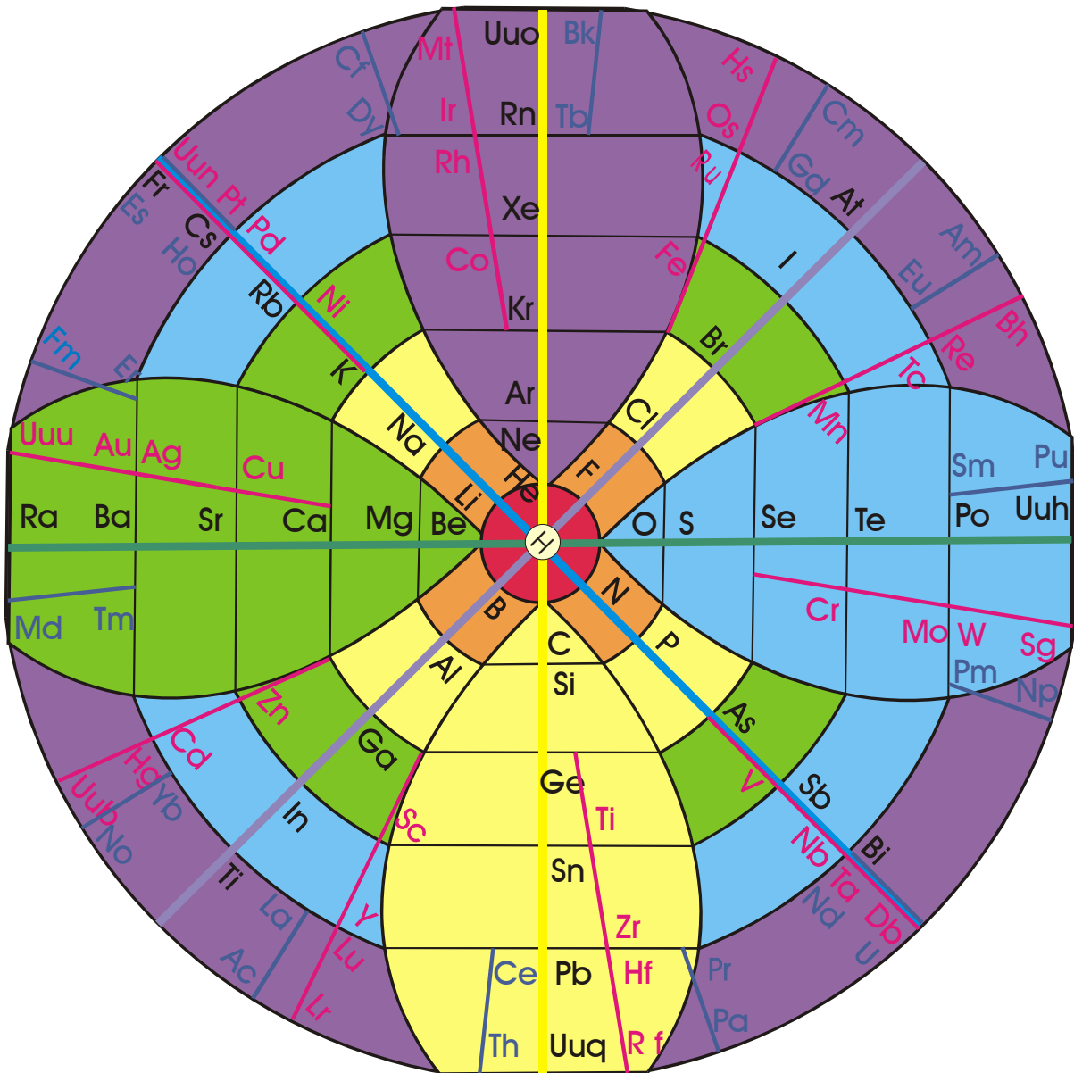
Gyroscopic Periodic Table orientated on the Internal Physical
